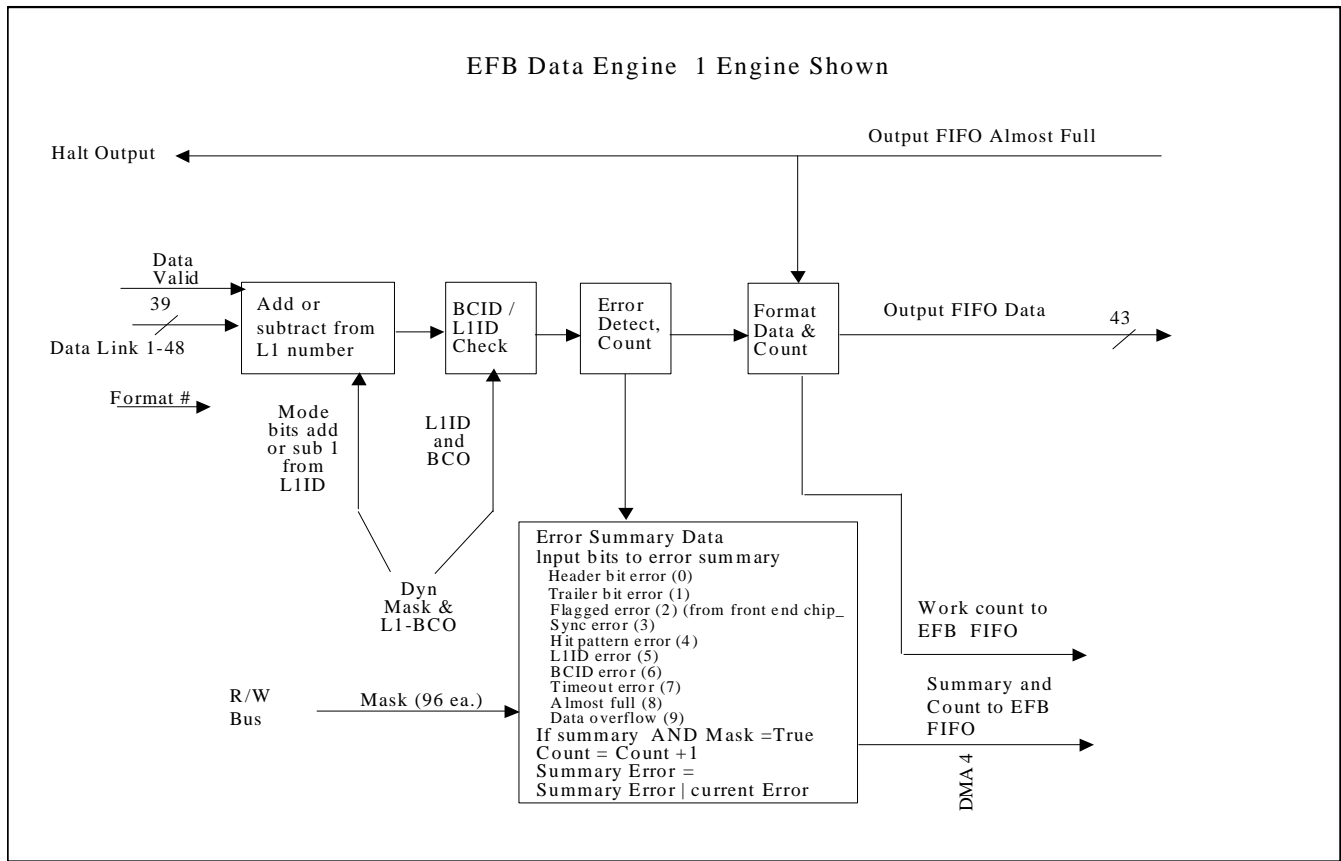
Figure 7: EFB data engine
