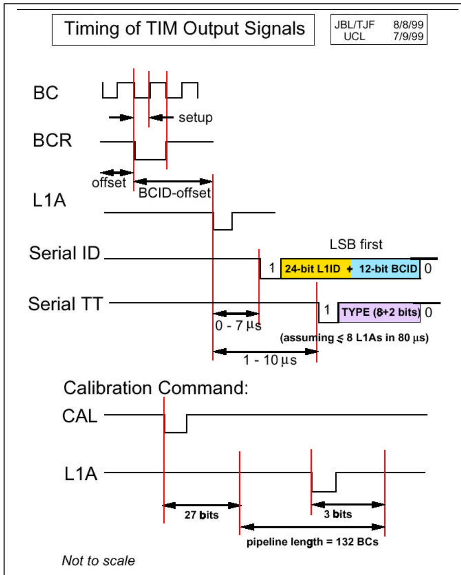
Figure 9: TIM to ROD Timing
